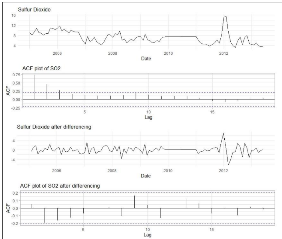
Figure 4. The time series plot for SO 2 and ACF before-after differencing.
