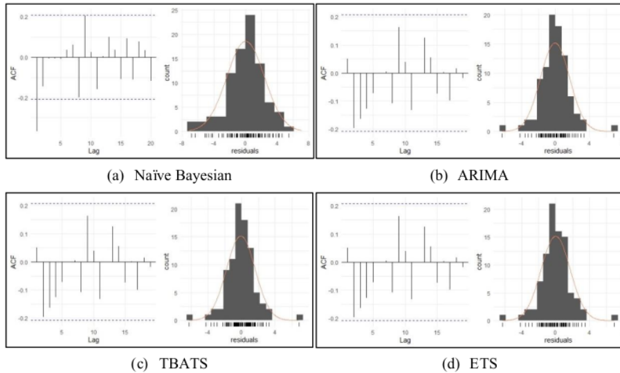
Figure 7. The ACF plot and histogram of models residual for SO 2 .
