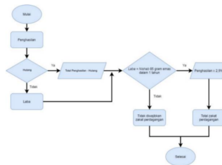
Gambar 4. Flowcart Sistem Perhitungan Zakat
