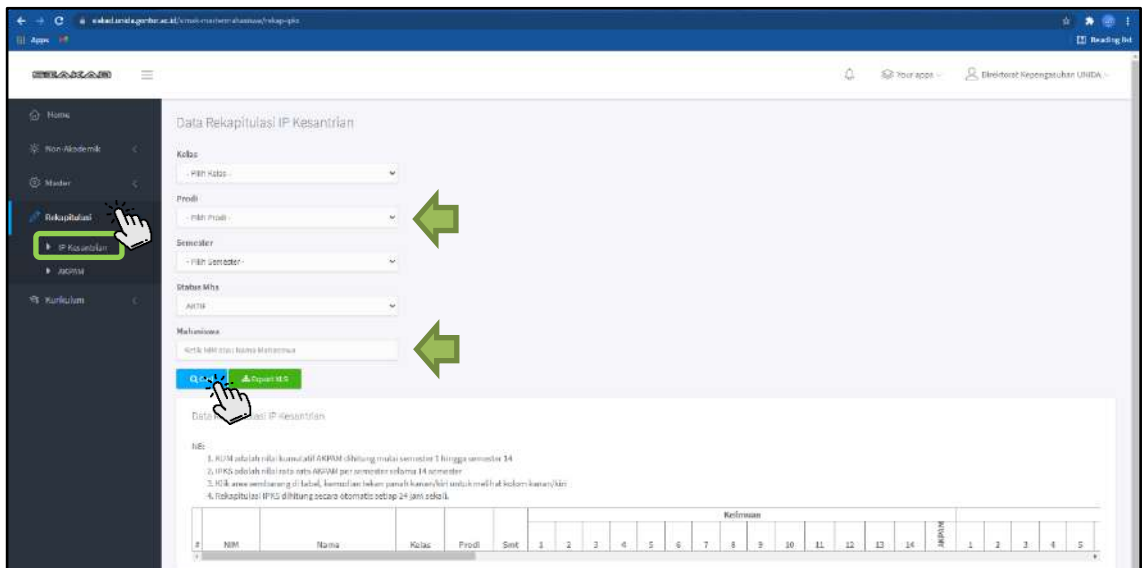
Gambar 2.34 IP Kesantrian
