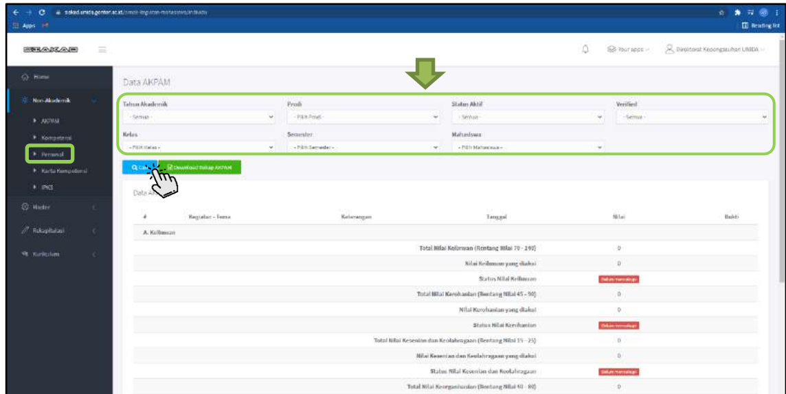
Gambar 2.13 Personal
