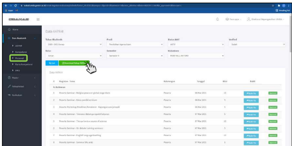
Gambar 2.14 Contoh Personal
