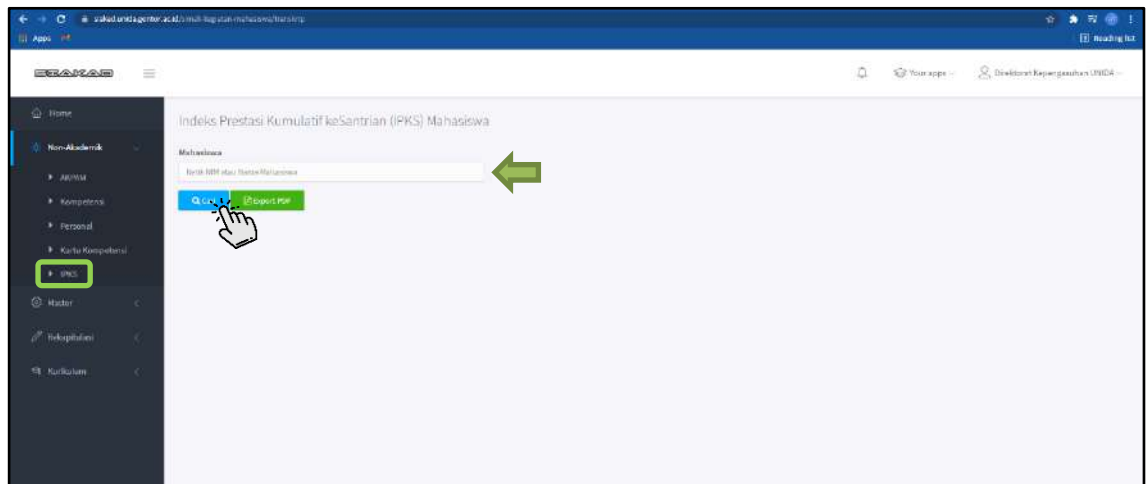
Gambar 2.18 IPKS
