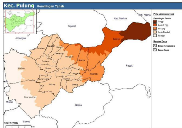
(a) Maps for land slope in Pulung
