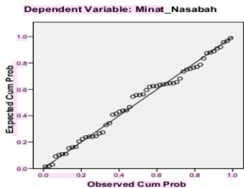
2 Normal P-P Plot of Regression Standardized Residual
