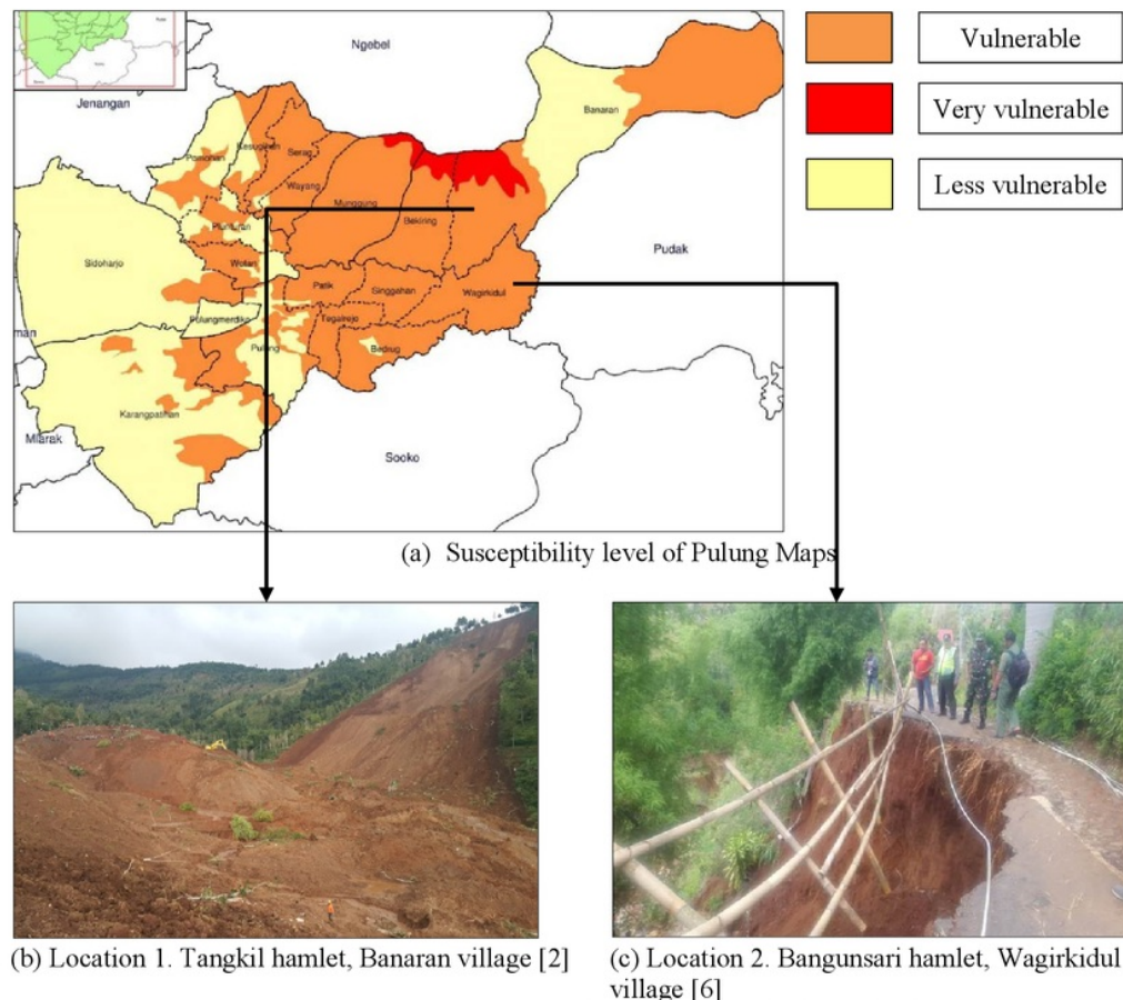
FIGURE 3. The landslide occurred in Banaran and Wagirkidul village
