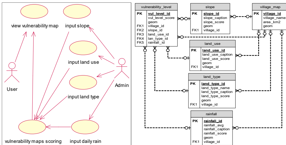
(a) Use Case Diagram of the proposed systems.
