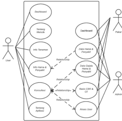
Gambar 1. Use case diagram sistem pakar
