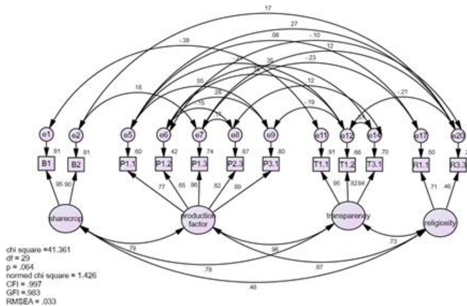
Figure 3 Path diagram measurement model
