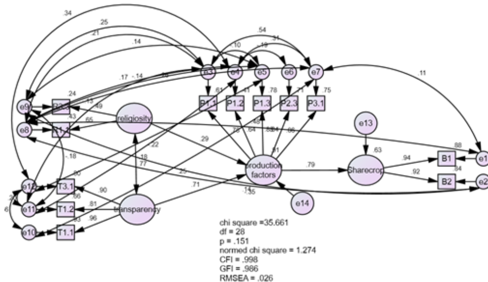
Figure 4 Path diagram structural model
