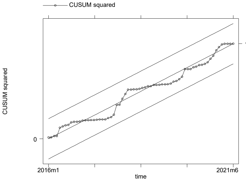
Figure 3. CUSUMQ Test for Stability
