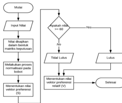
Gambar 2. Flowchart proses perhitungan nilai
